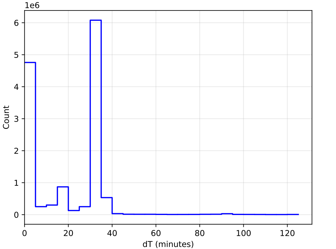
too_elab_heavy_r64_d2_ugrizy_v3.4_10yrs All sky: DeltaT Histogram
