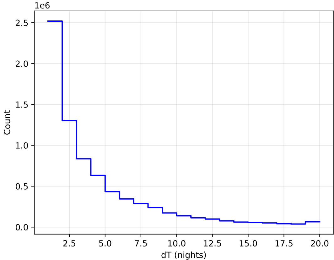
too_elab_heavy_r64_d2_ugrizy_v3.4_10yrs WFD all bands: DeltaNight Histogram
