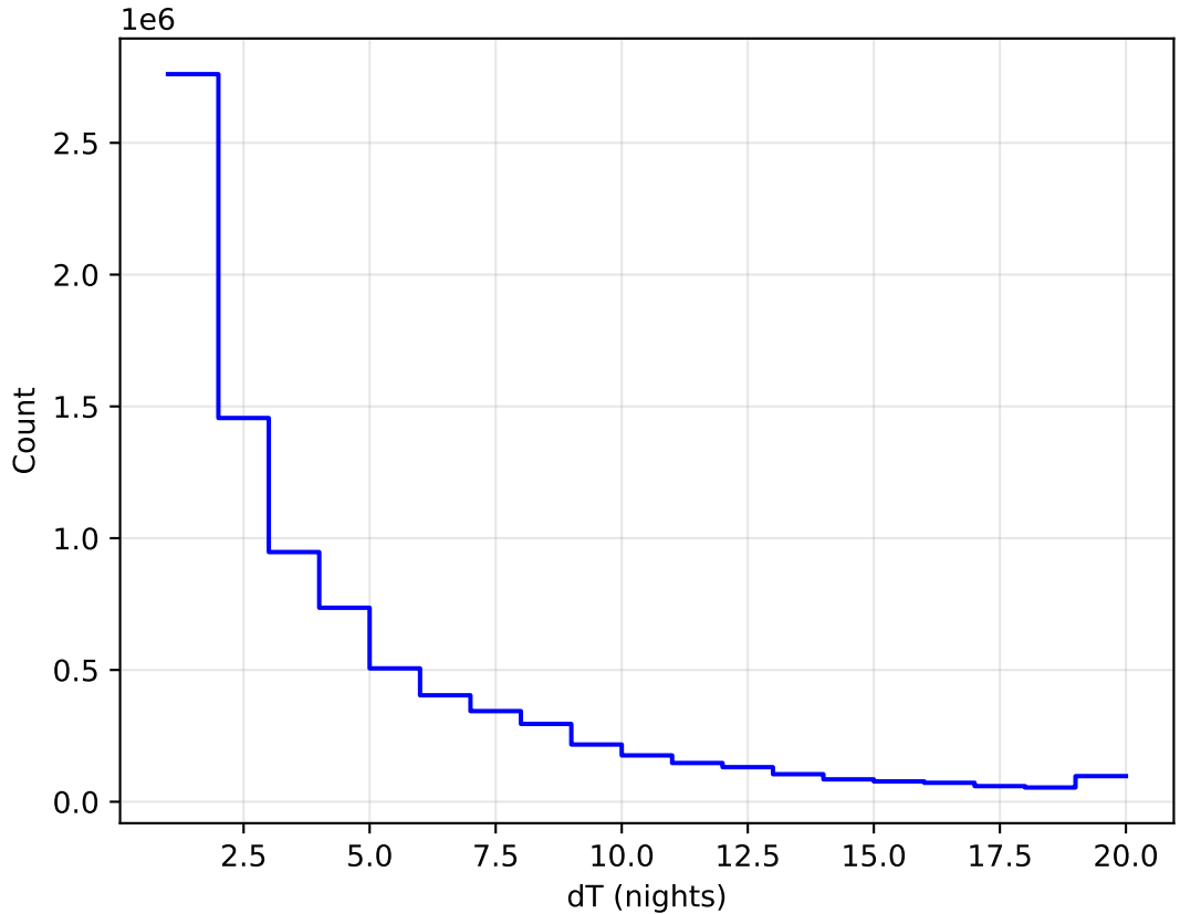
too_elab_heavy_r64_d2_ugrizy_v3.4_10yrs All sky all bands: DeltaNight Histogram
