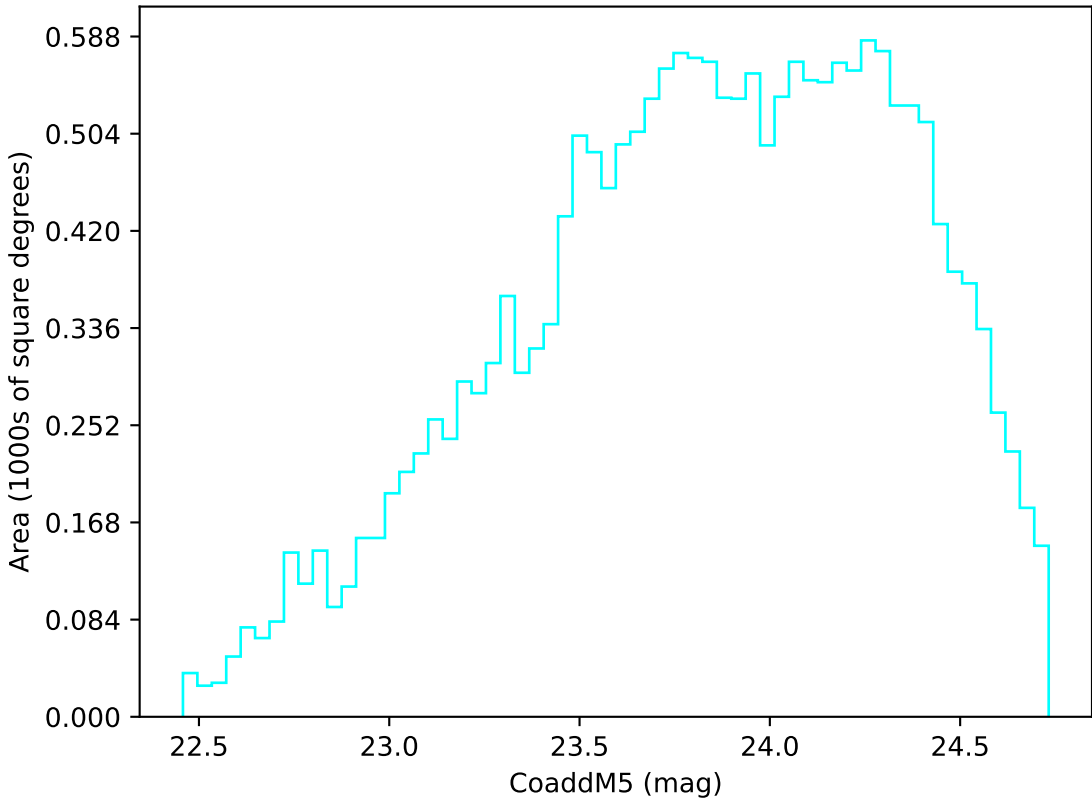
too_elab_heavy_r64_d2_ugrizy_v3.4_10yrs Yr 3-4 u band: CoaddM5
