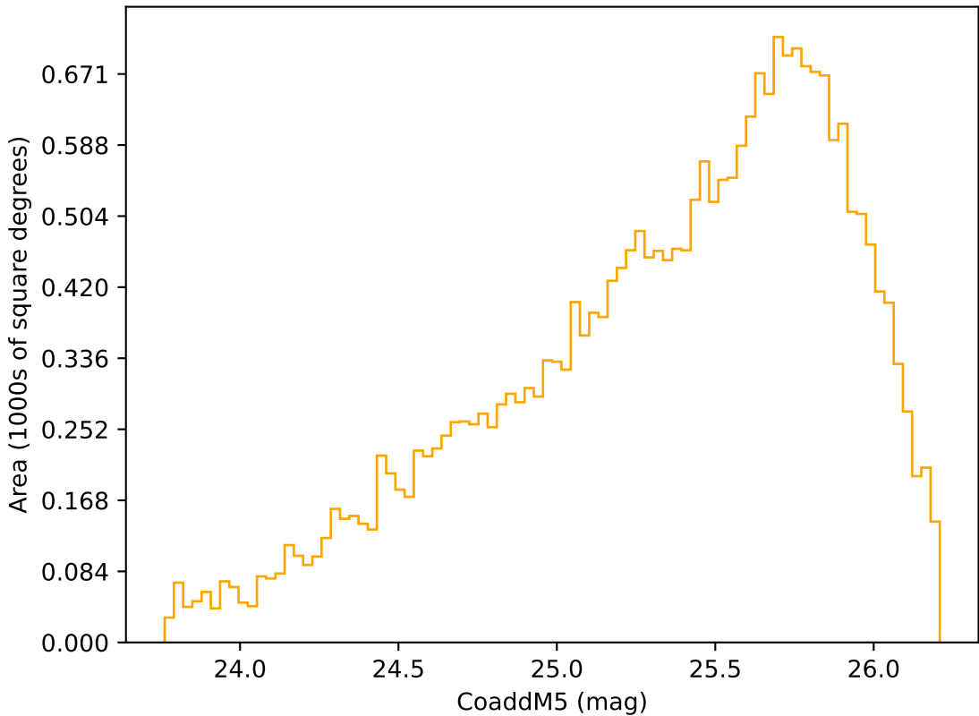
too_elab_heavy_r64_d2_ugrizy_v3.4_10yrs Yr 3-4 r band: CoaddM5
