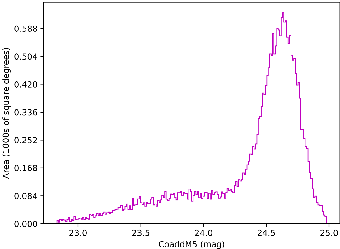
too_elab_heavy_r64_d2_ugrizy_v3.4_10yrs Yr 1 z band: CoaddM5
