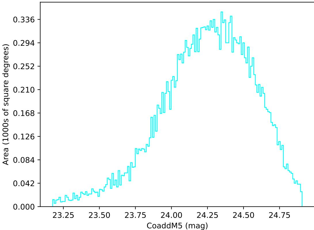
too_elab_heavy_r64_d2_ugrizy_v3.4_10yrs Yr 1 u band: CoaddM5
