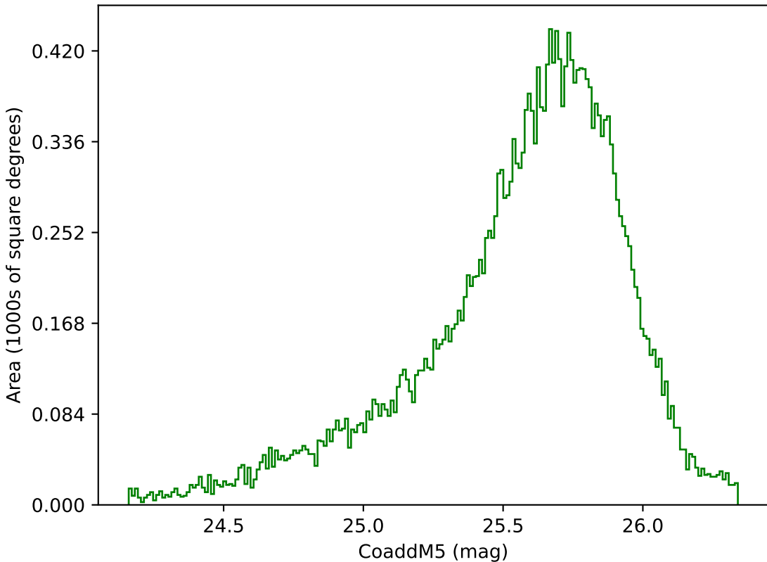
too_elab_heavy_r64_d2_ugrizy_v3.4_10yrs Yr 1 g band: CoaddM5
