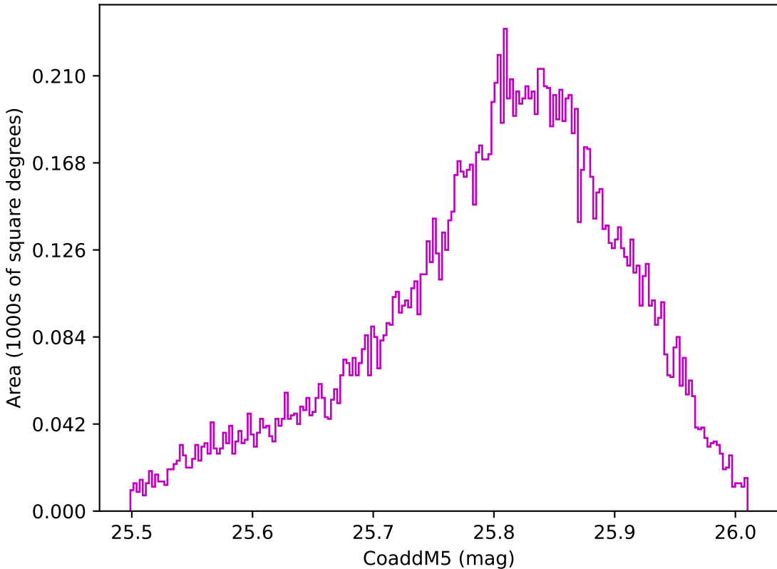
too_elab_heavy_r64_d2_ugrizy_v3.4_10yrs WFD z band: CoaddM5
