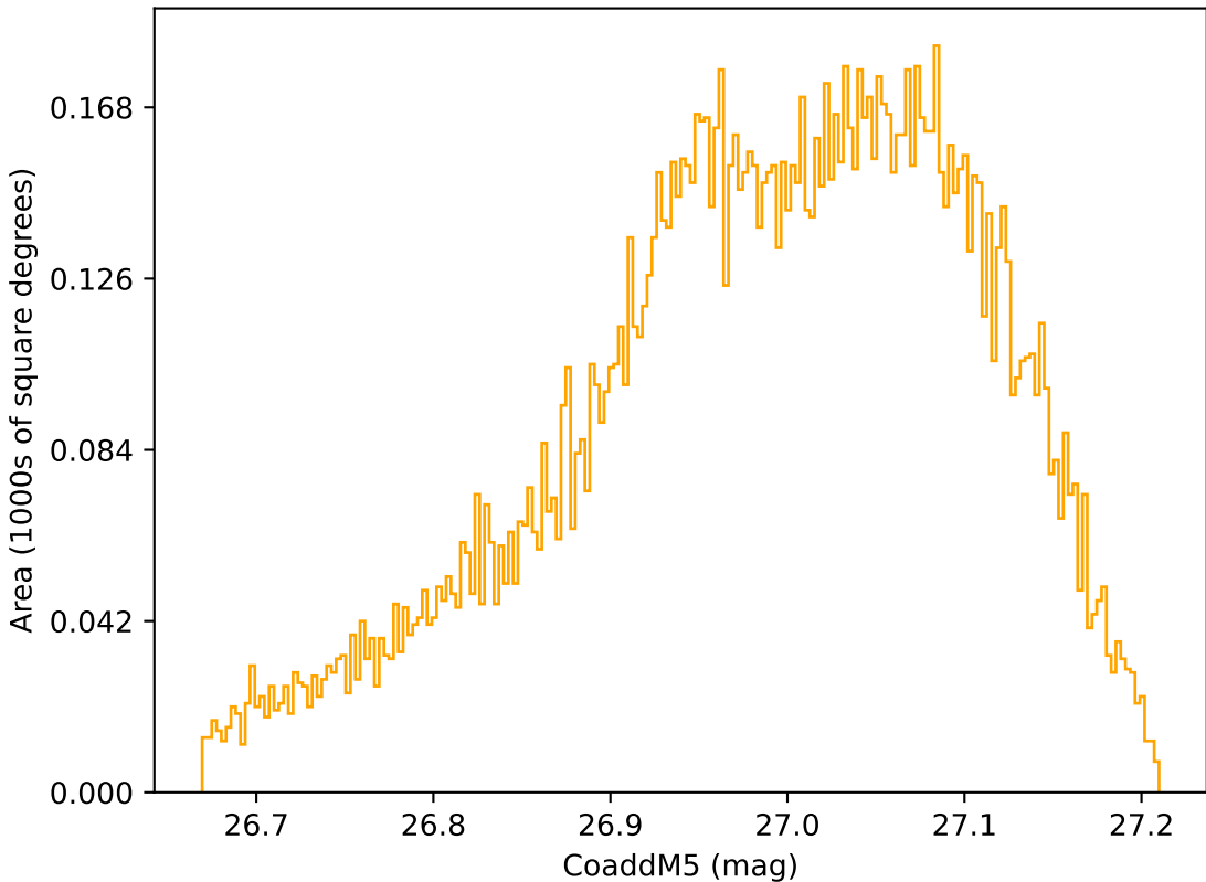
too_elab_heavy_r64_d2_ugrizy_v3.4_10yrs WFD r band: CoaddM5
