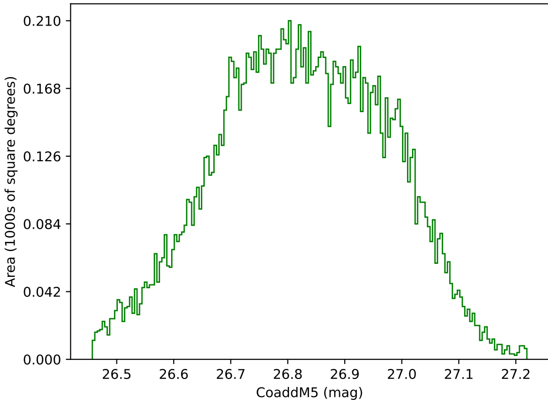
too_elab_heavy_r64_d2_ugrizy_v3.4_10yrs WFD g band: CoaddM5
