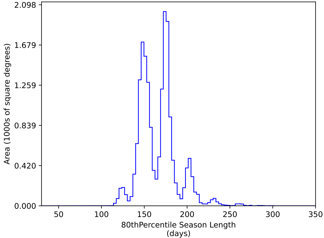
too_elab_heavy_r64_d2_ugrizy_v3.4_10yrs WFD y band: 80thPercentile Season Length
