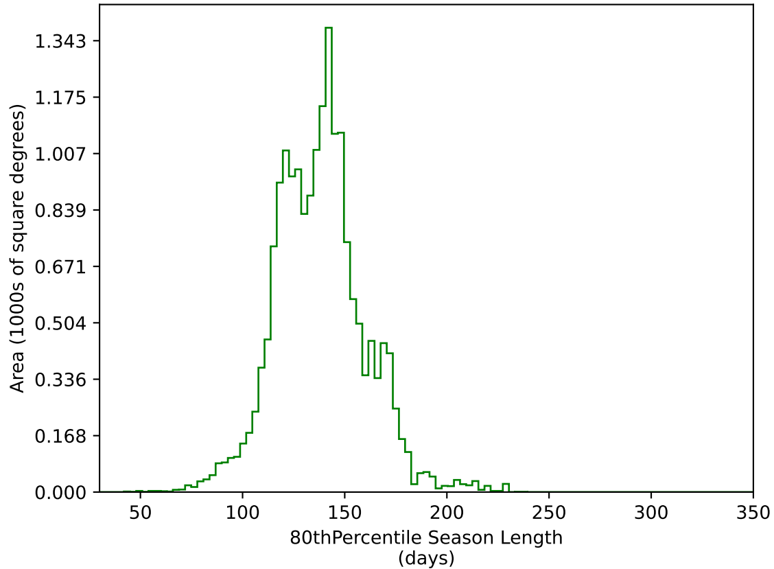
too_elab_heavy_r64_d2_ugrizy_v3.4_10yrs WFD g band: 80thPercentile Season Length
