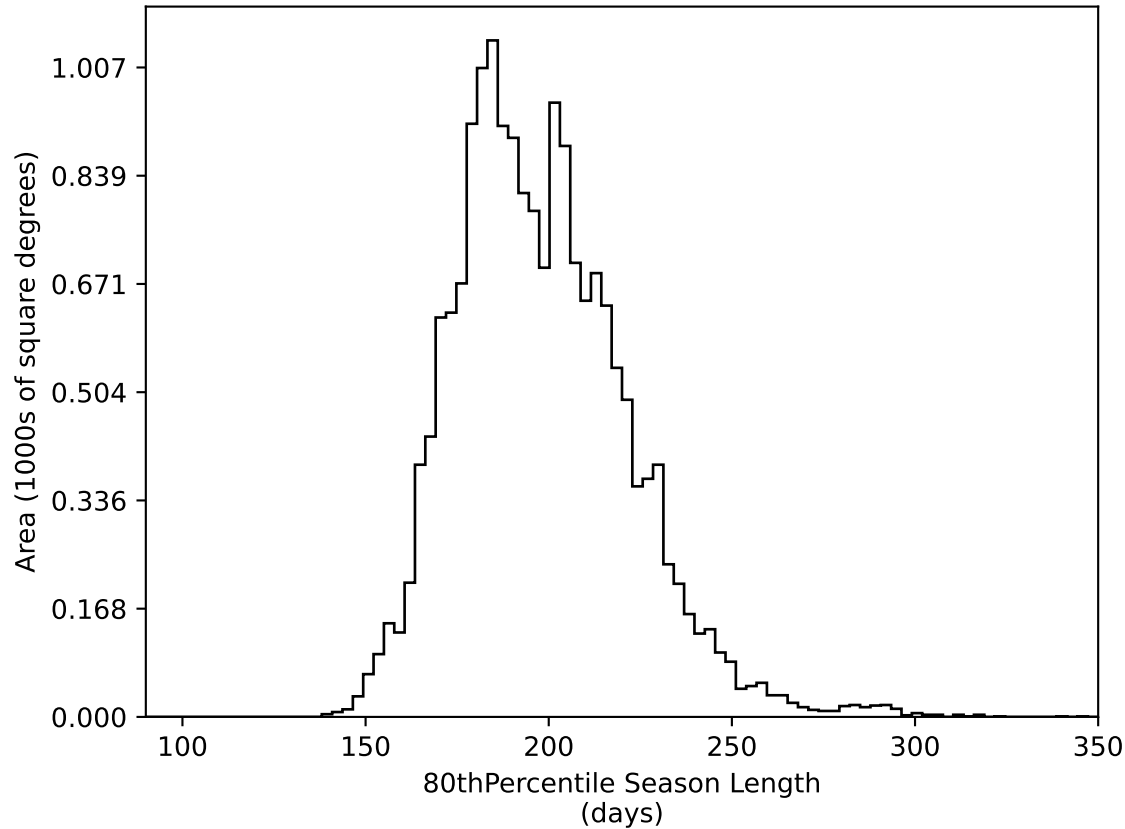
too_elab_heavy_r64_d2_ugrizy_v3.4_10yrs WFD all bands: 80thPercentile Season Length
