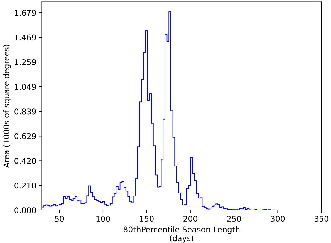
too_elab_heavy_r64_d2_ugrizy_v3.4_10yrs All sky y band: 80thPercentile Season Length
