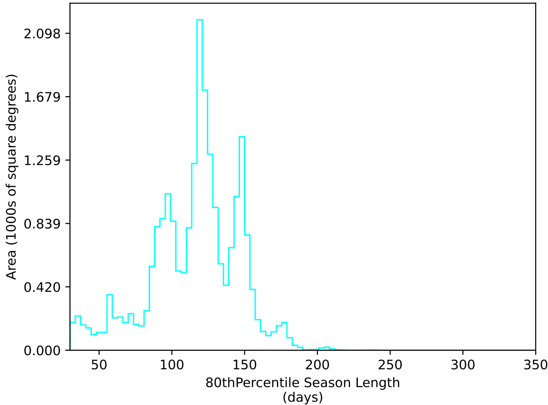
too_elab_heavy_r64_d2_ugrizy_v3.4_10yrs All sky u band: 80thPercentile Season Length
