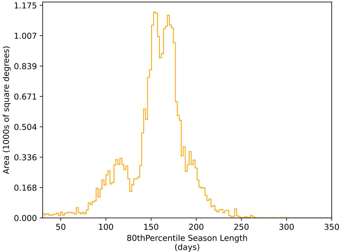
too_elab_heavy_r64_d2_ugrizy_v3.4_10yrs All sky r band: 80thPercentile Season Length
