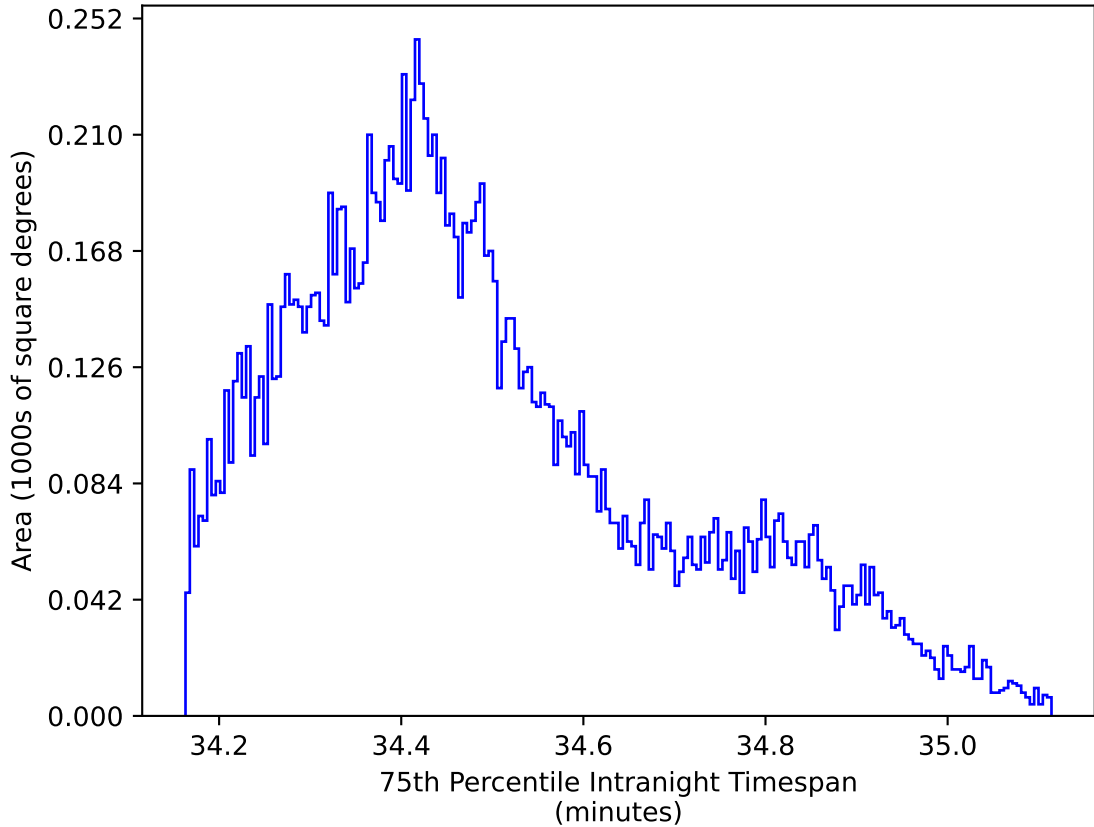
too_elab_heavy_r64_d2_ugrizy_v3.4_10yrs WFD zy bands: 75th Percentile Intranight Timespan
