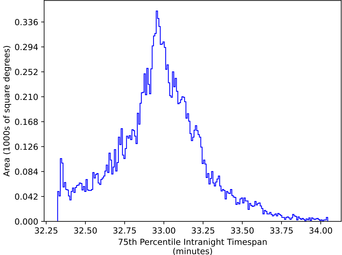
too_elab_heavy_r64_d2_ugrizy_v3.4_10yrs WFD y band: 75th Percentile Intranight Timespan
