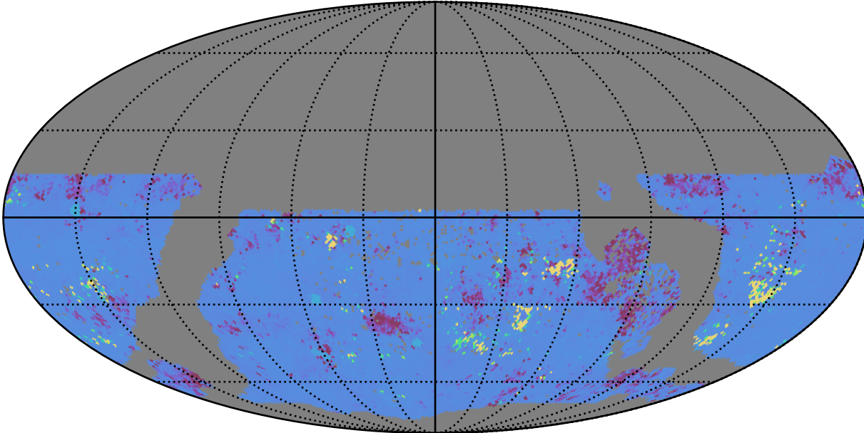
too_elab_heavy_r64_d2_ugrizy_v3.4_10yrs WFD ug bands: 75th Percentile Intranight Timespan
