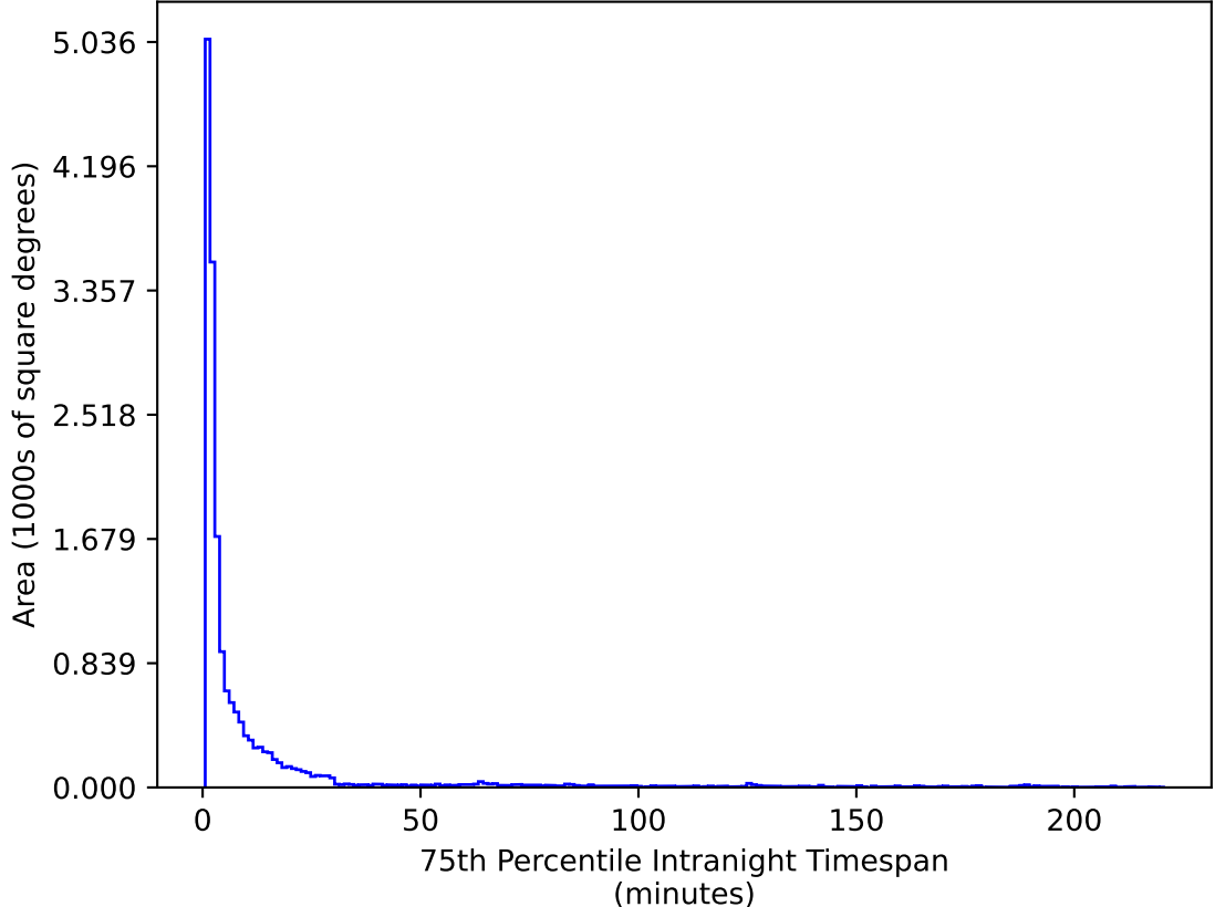
too_elab_heavy_r64_d2_ugrizy_v3.4_10yrs_WFD_u_band: 75th Percentile Intranight Timespan
