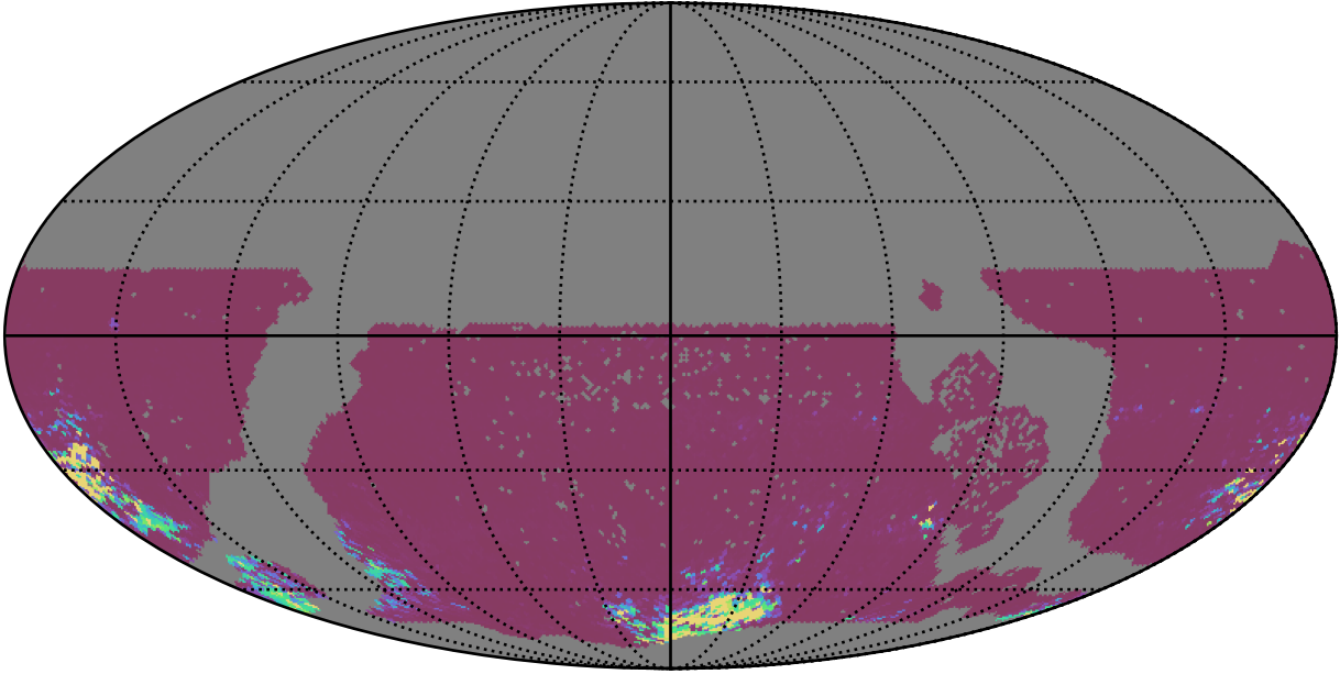
too_elab_heavy_r64_d2_ugrizy_v3.4_10yrs WFD ri bands: 75th Percentile Intranight Timespan
