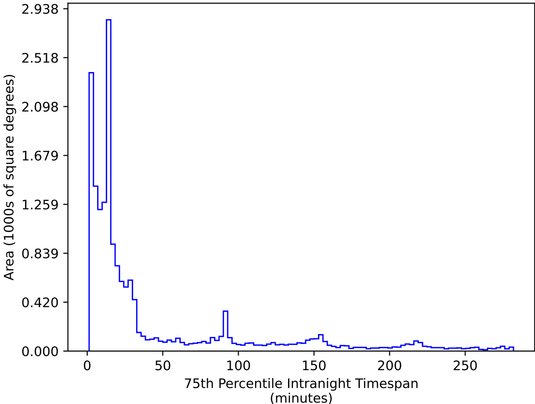
too_elab_heavy_r64_d2_ugrizy_v3.4_10yrs WFD r band: 75th Percentile Intranight Timespan
