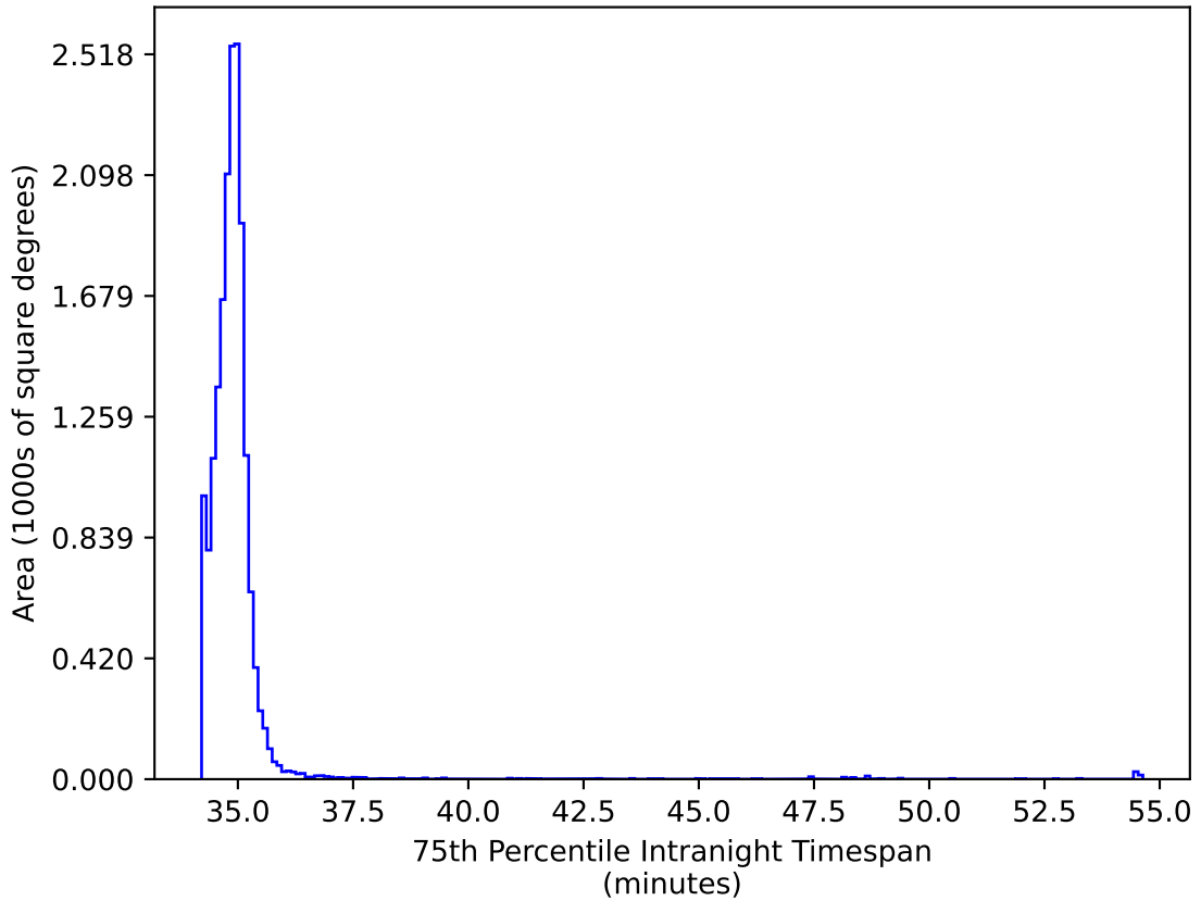
too_elab_heavy_r64_d2_ugrizy_v3.4_10yrs WFD iz bands: 75th Percentile Intranight Timespan
