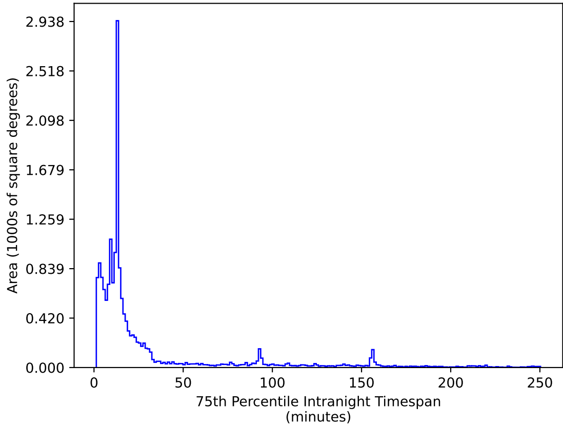
too_elab_heavy_r64_d2_ugrizy_v3.4_10yrs WFD i band: 75th Percentile Intranight Timespan
