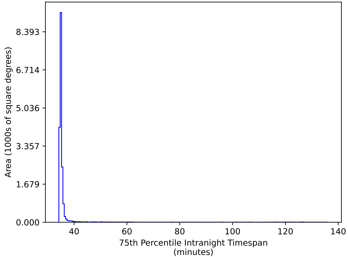
too_elab_heavy_r64_d2_ugrizy_v3.4_10yrs WFD gr bands: 75th Percentile Intranight Timespan
