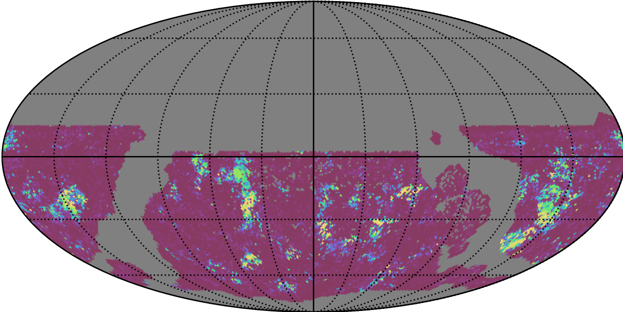
too_elab_heavy_r64_d2_ugrizy_v3.4_10yrs WFD g band: 75th Percentile Intranight Timespan
