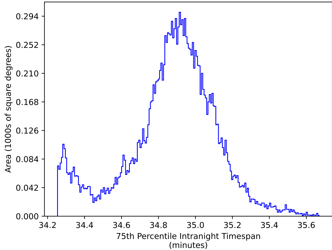
too_elab_heavy_r64_d2_ugrizy_v3.4_10yrs WFD all bands: 75th Percentile Intranight Timespan
