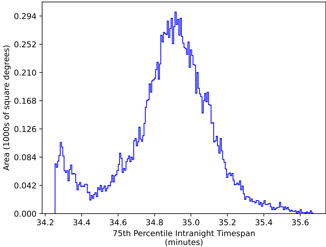
too_elab_heavy_r64_d2_ugrizy_v3.4_10yrs WFD: 75th Percentile Intranight Timespan
