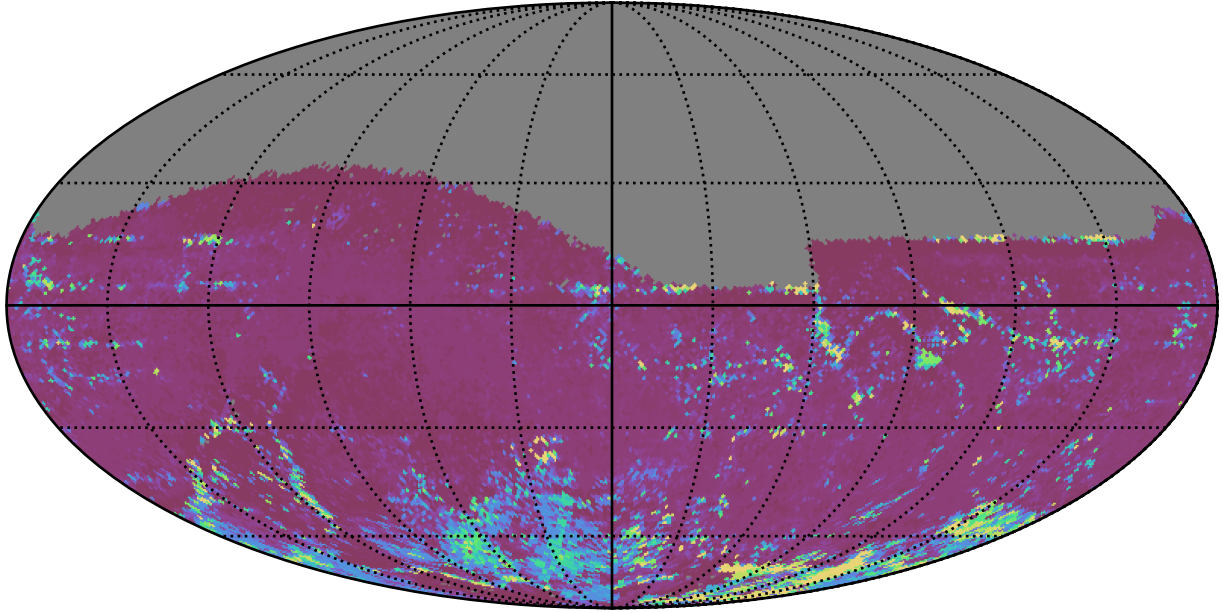
too_elab_heavy_r64_d2_ugrizy_v3.4_10yrs All sky z band: 75th Percentile Intranight Timespan
