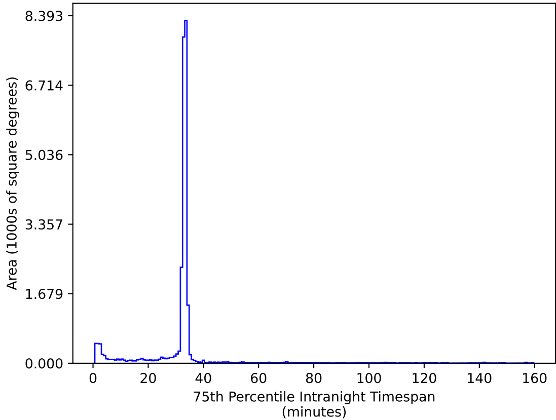
too_elab_heavy_r64_d2_ugrizy_v3.4_10yrs All sky ug bands: 75th Percentile Intranight Timespan
