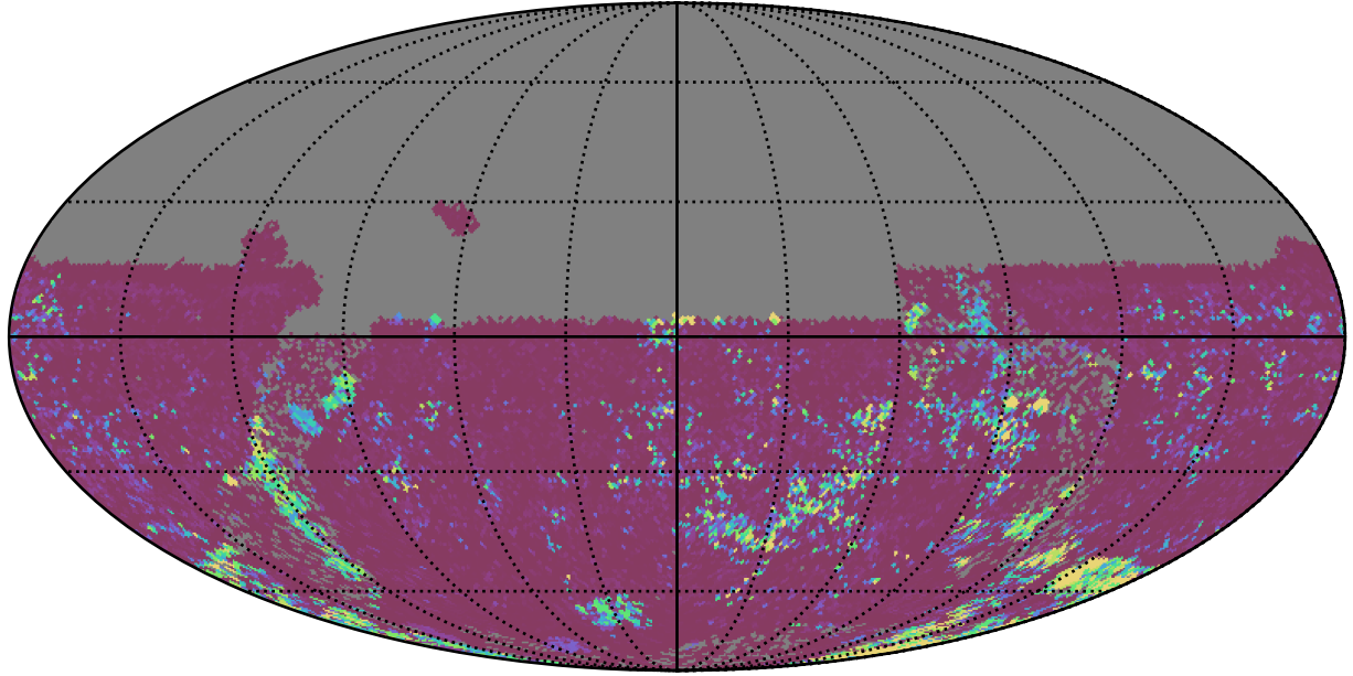
too_elab_heavy_r64_d2_ugrizy_v3.4_10yrs All sky u band: 75th Percentile Intranight Timespan
