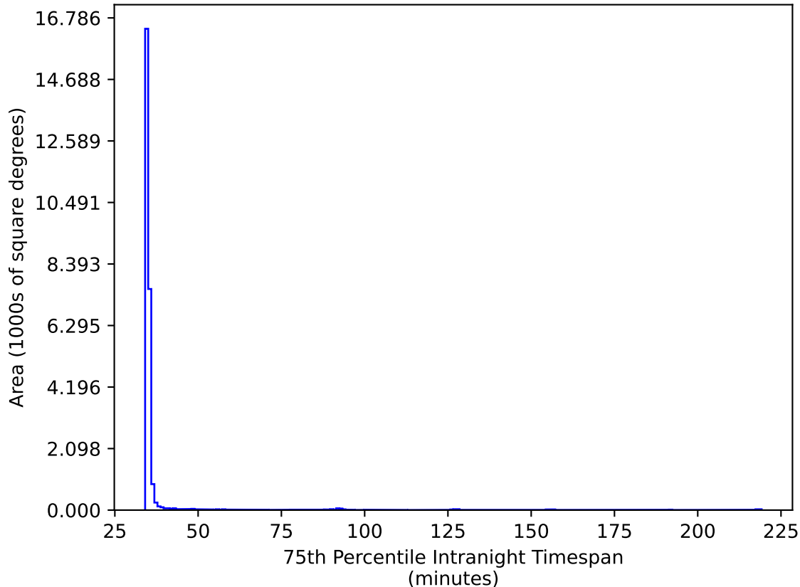
too_elab_heavy_r64_d2_ugrizy_v3.4_10yrs All sky ri bands: 75th Percentile Intranight Timespan
