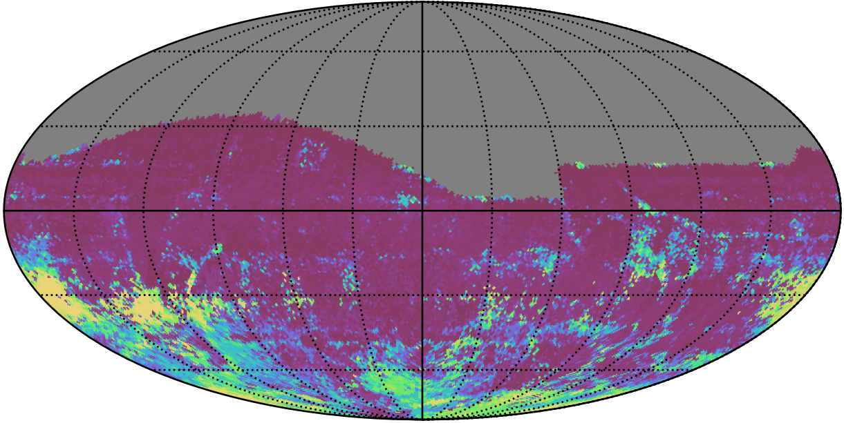
too_elab_heavy_r64_d2_ugrizy_v3.4_10yrs All sky r band: 75th Percentile Intranight Timespan
