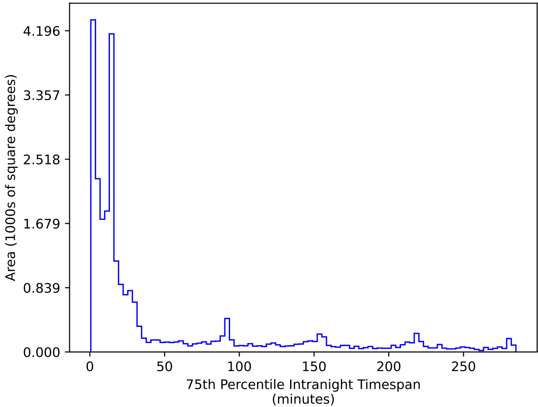
too_elab_heavy_r64_d2_ugrizy_v3.4_10yrs All sky r band: 75th Percentile Intranight Timespan
