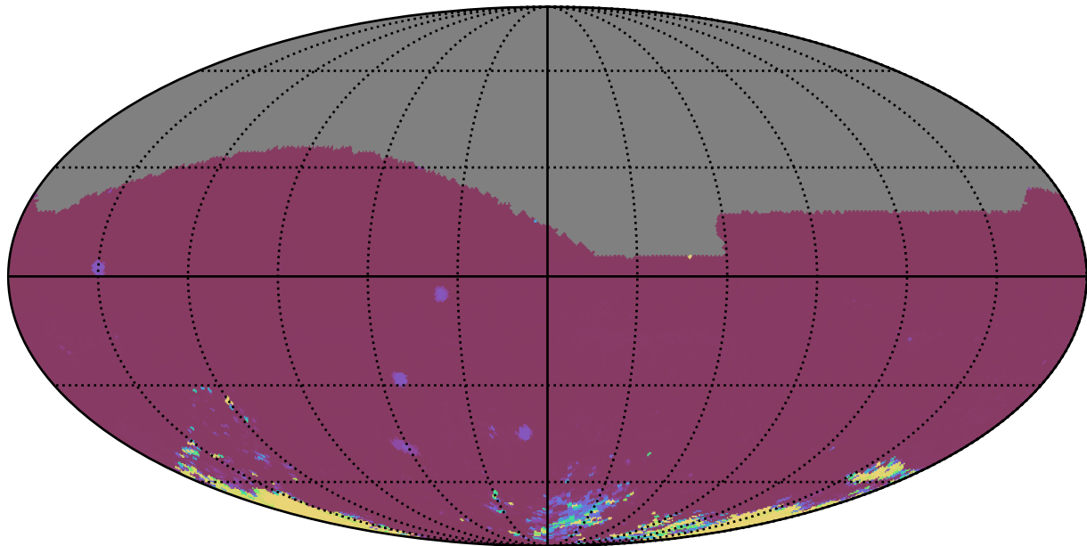
too_elab_heavy_r64_d2_ugrizy_v3.4_10yrs All sky iz bands: 75th Percentile Intranight Timespan
