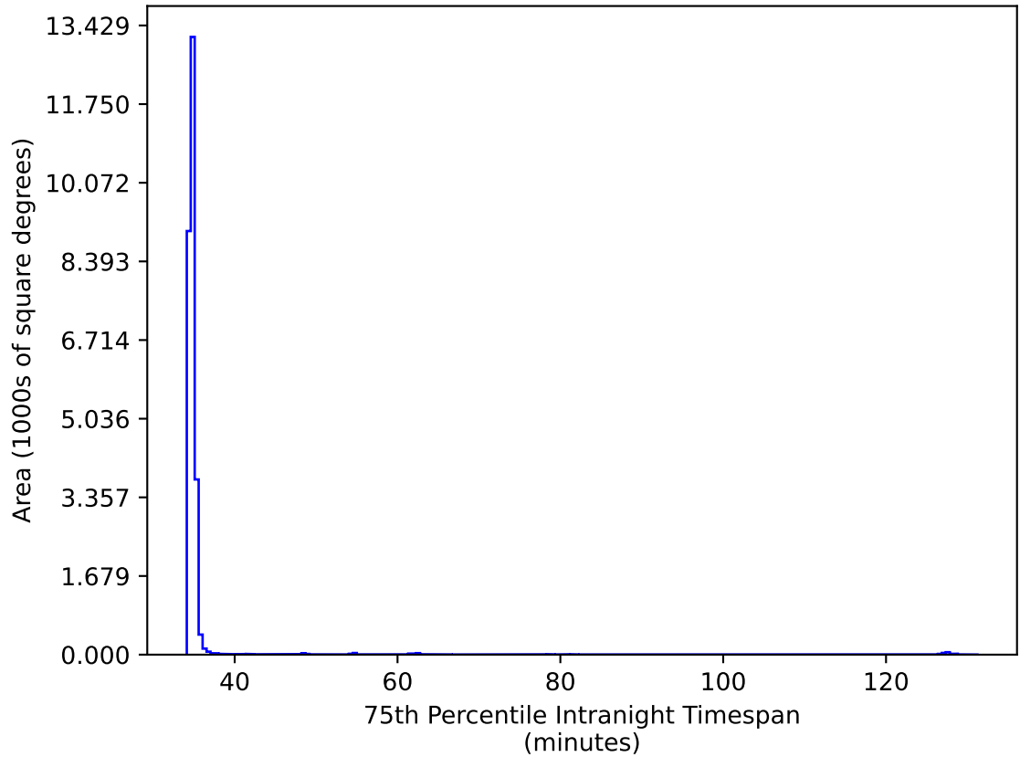
too_elab_heavy_r64_d2_ugrizy_v3.4_10yrs All sky iz bands: 75th Percentile Intranight Timespan
