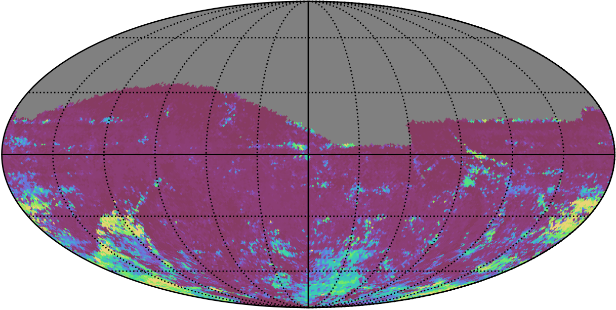
too_elab_heavy_r64_d2_ugrizy_v3.4_10yrs All sky i band: 75th Percentile Intranight Timespan
