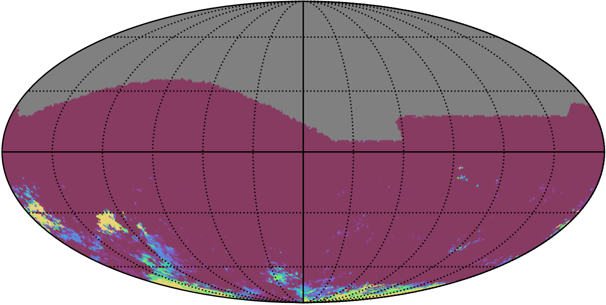
too_elab_heavy_r64_d2_ugrizy_v3.4_10yrs All sky gr bands: 75th Percentile Intranight Timespan
