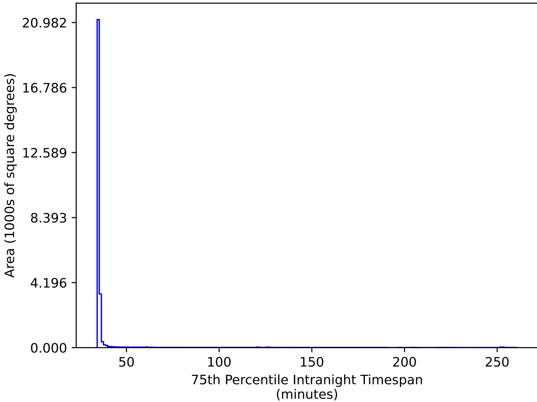
too_elab_heavy_r64_d2_ugrizy_v3.4_10yrs All sky gr bands: 75th Percentile Intranight Timespan
