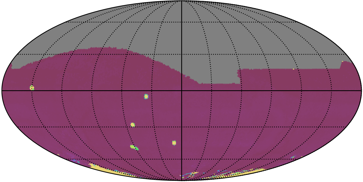
too_elab_heavy_r64_d2_ugrizy_v3.4_10yrs All sky all bands: 75th Percentile Intranight Timespan
