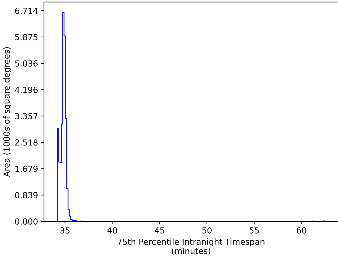
too_elab_heavy_r64_d2_ugrizy_v3.4_10yrs All sky all bands: 75th Percentile Intranight Timespan
