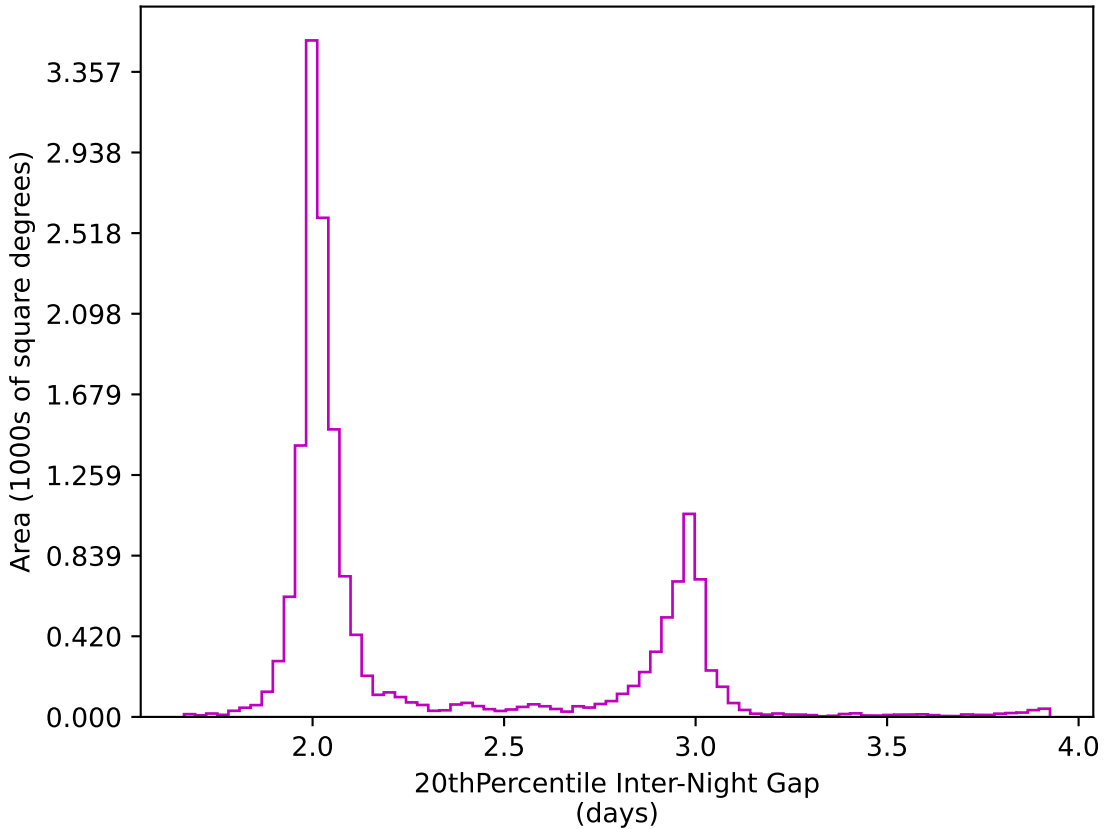
too_elab_heavy_r64_d2_ugrizy_v3.4_10yrs WFD z band: 20thPercentile Inter-Night Gap
