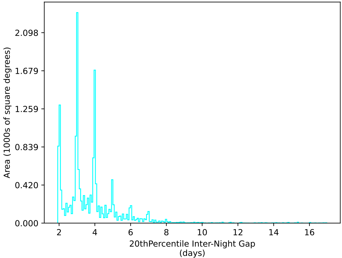
too_elab_heavy_r64_d2_ugrizy_v3.4_10yrs WFD u band: 20thPercentile Inter-Night Gap
