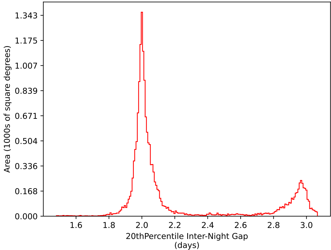
too_elab_heavy_r64_d2_ugrizy_v3.4_10yrs WFD i band: 20thPercentile Inter-Night Gap
