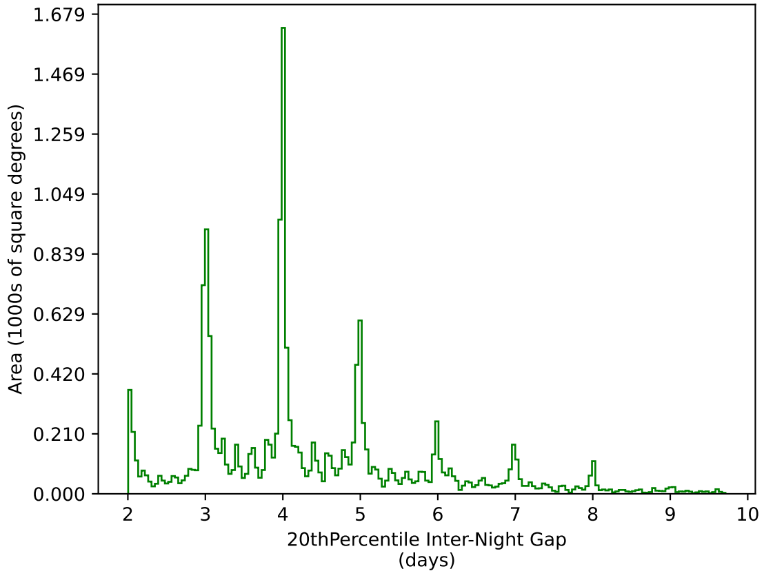
too_elab_heavy_r64_d2_ugrizy_v3.4_10yrs WFD g band: 20thPercentile Inter-Night Gap
