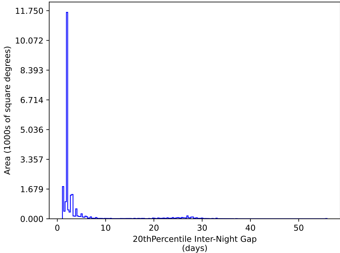
too_elab_heavy_r64_d2_ugrizy_v3.4_10yrs All sky y band: 20thPercentile Inter-Night Gap
