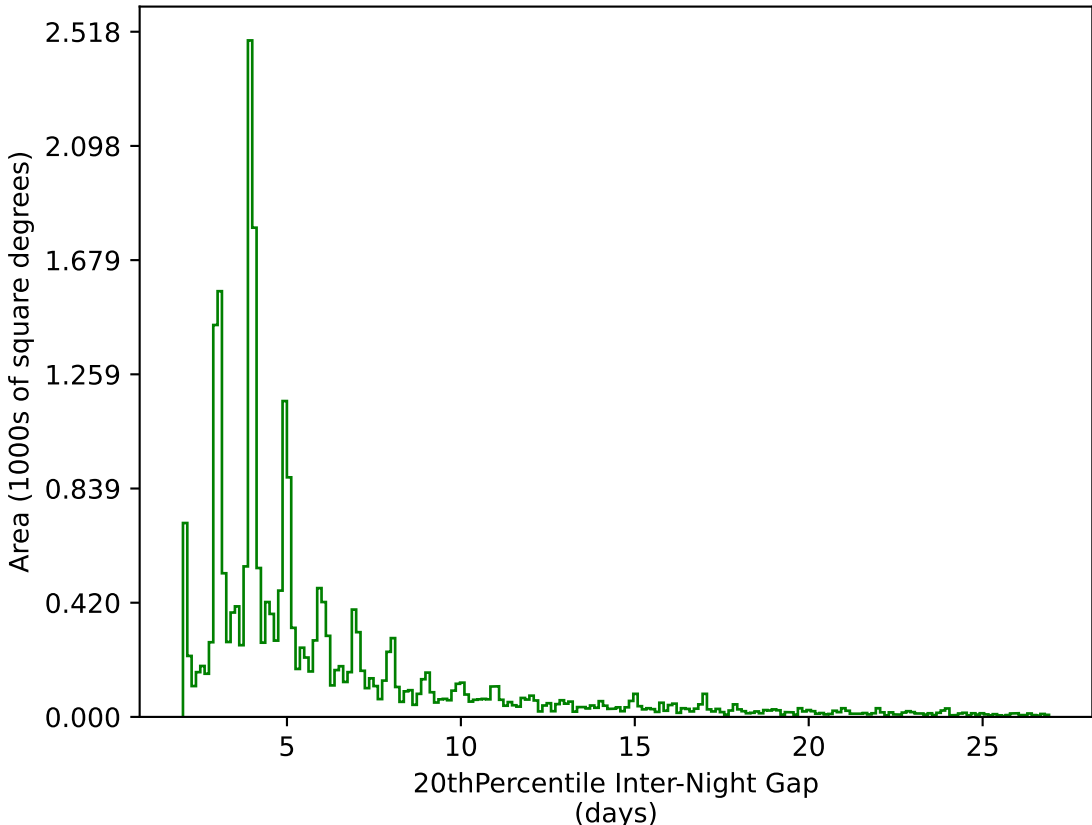
too_elab_heavy_r64_d2_ugrizy_v3.4_10yrs All sky g band: 20thPercentile Inter-Night Gap
