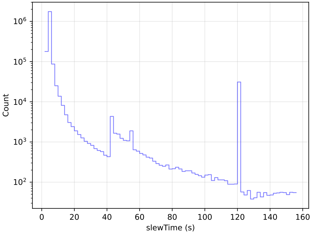
too_elab_heavy_r64_d2_ugrizy_v3.4_10yrs All visits: Slew Time Histogram
