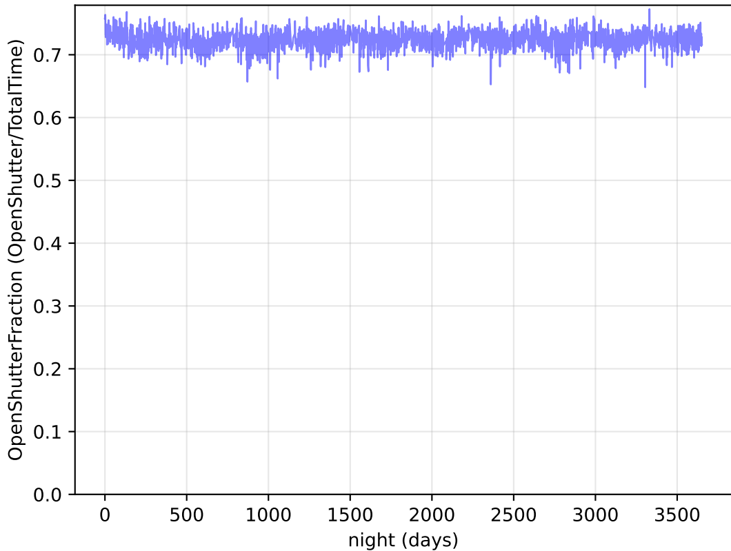
too_elab_heavy_r64_d2_ugrizy_v3.4_10yrs : OpenShutterFraction
